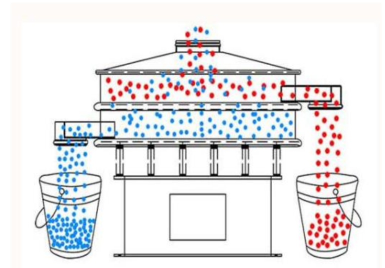
Vibrating Screen
